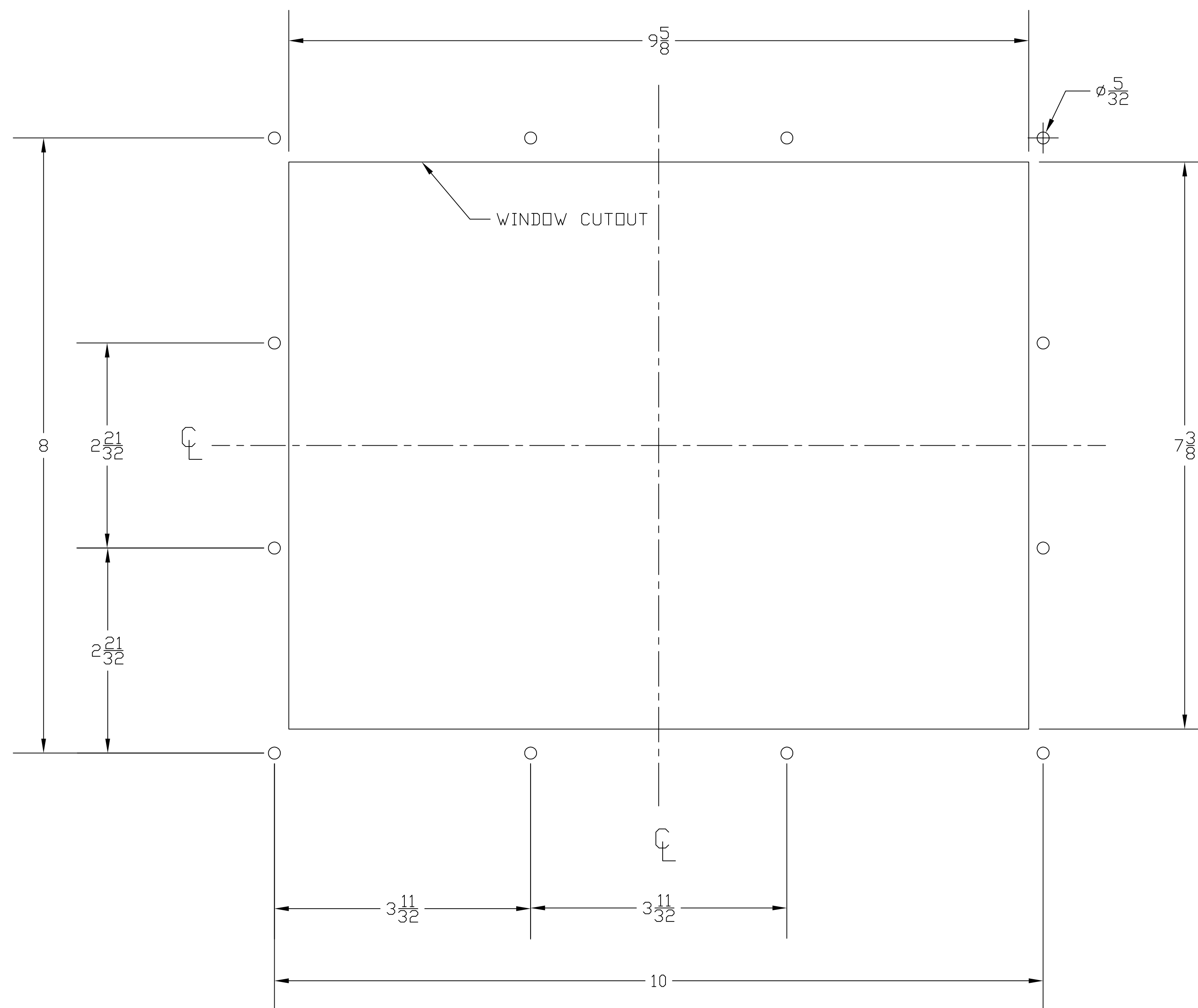
MOUNTING DETAIL
